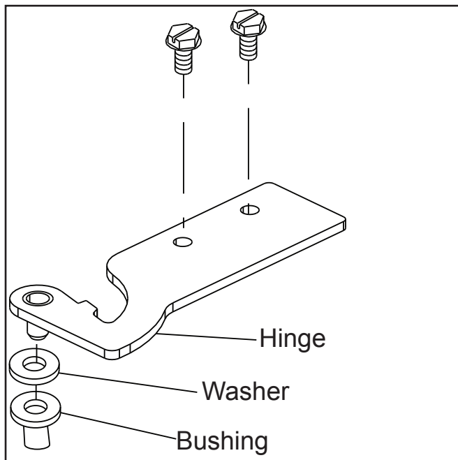
Installation on original production door.
