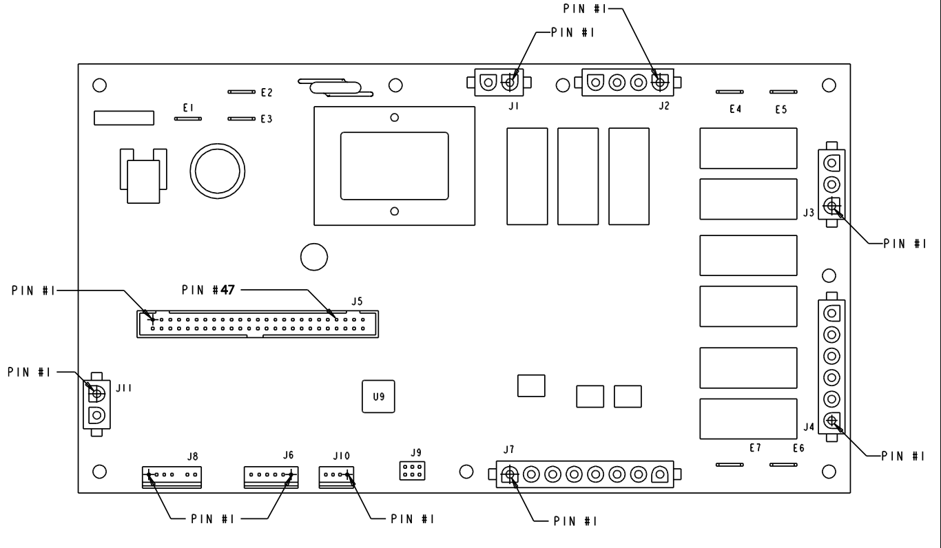
H.V. Board – Connector Locations
