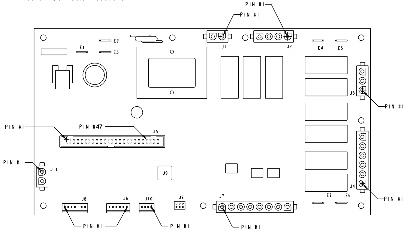
H.V. Board – Connector Locations
